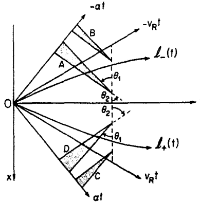
Fig. 3. Regions of integration for the determination of F_{\pm} and G_{\pm} . Triangles A, B identify the regions of integration for the integral in (2.6a) for x \geq l_{-}(t) respectively while C and D identify the regions of integration for the integral in (2.6b) for x \geq l_{+}(t) . The angles \theta_1 = \tan^{-1}(\alpha^{-1}) and \theta_2 = \tan^{-1}(\beta^{-1}) .
