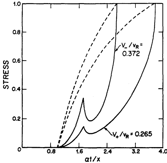
Fig. 6. Exact (solid) and approximate (dashed) stress distribution scaled with respect to the stresses at the edges of the crack for self-similar in-plane propagation. V_+/v_R = 0.265 and V_-/v_R = 0.372 . The cusps in the exact solution are due to the discontinuous derivatives at the S-wave front.
